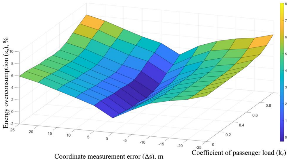
Fig. 10. Dependency of energy overconsumption \epsilon_A on error of measurement of train coordinate and train weight deviations for type III ('heavy') gradient profile
